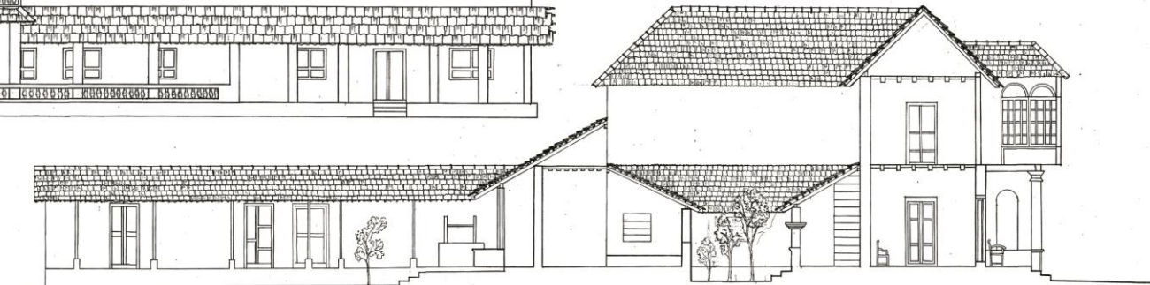
SECTION BB
